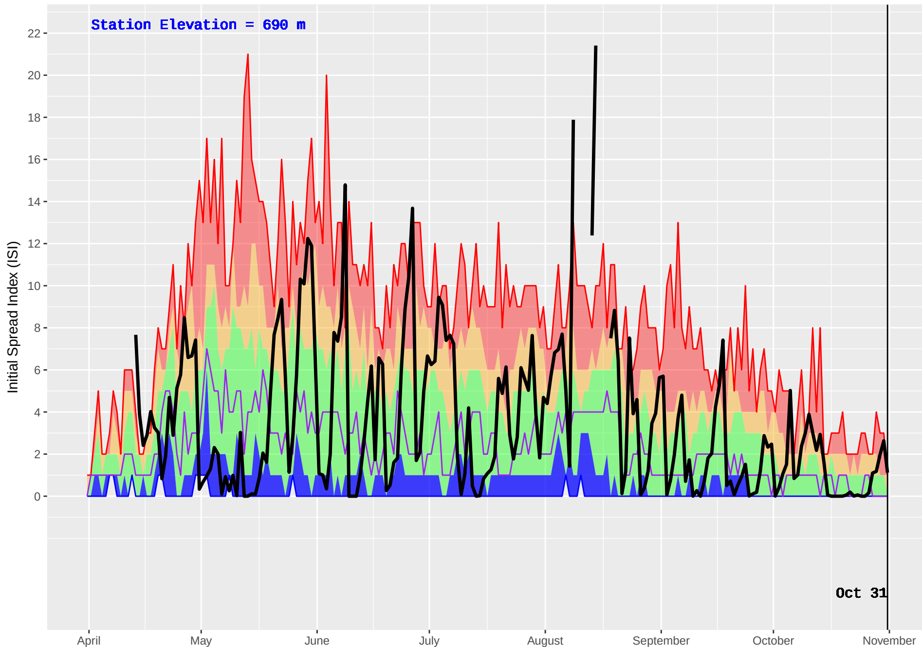
MACKENZIE FS (155) : Historical (1994–2016) and Current (2017) Noon Initial Spread Index (ISI)
