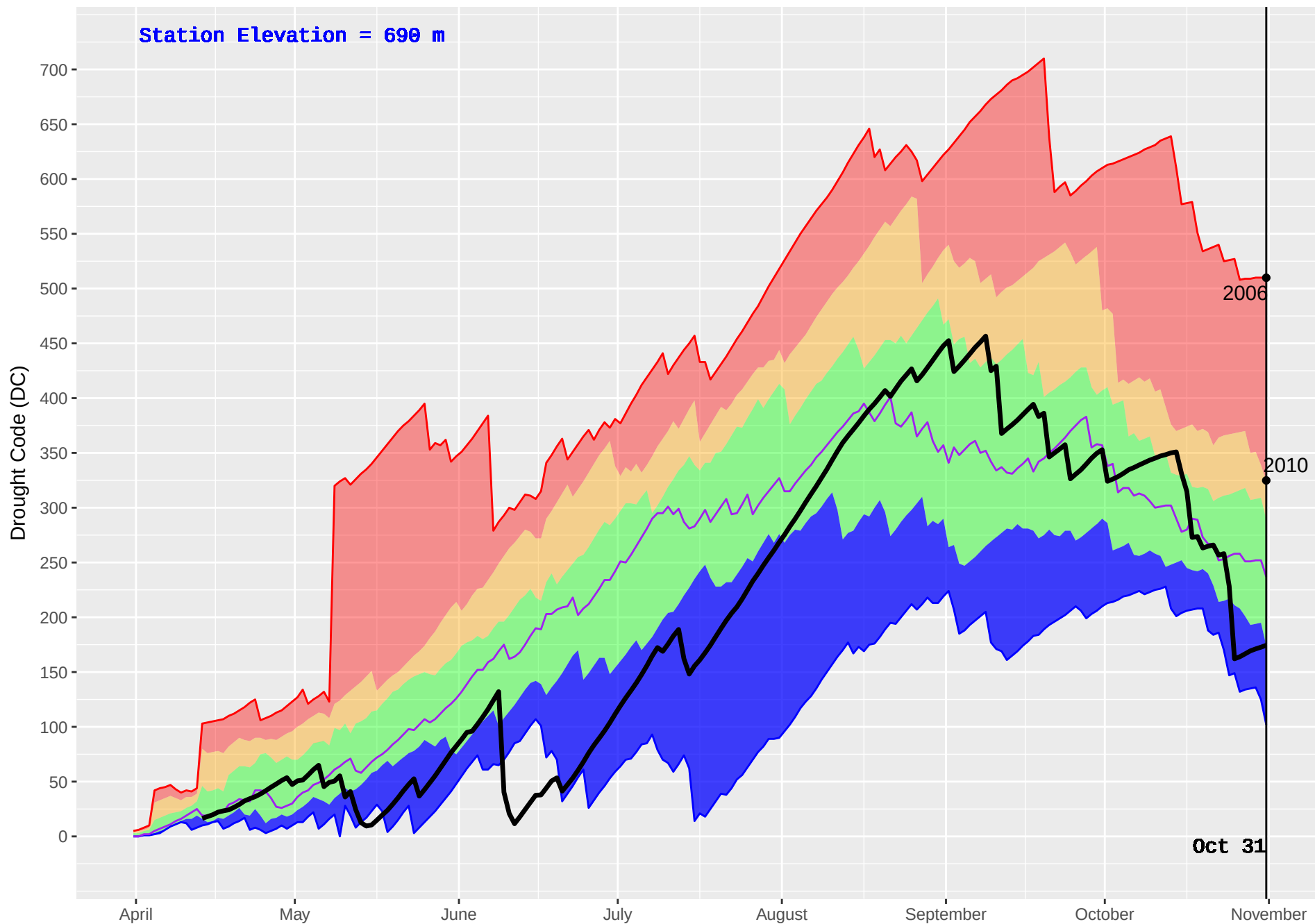
MACKENZIE FS (155) : Historical (1994–2016) and Current (2017) Noon Drought Code (DC)
